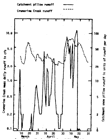
Fig. 5. Runoff from the Catchment Snow Pillow and from Crumrine Creek. March-May 1970
