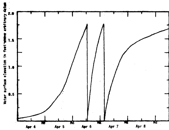
Figure 3. Trace of water surface elevation in the drain tanks for April 4 to 6, 1970.
