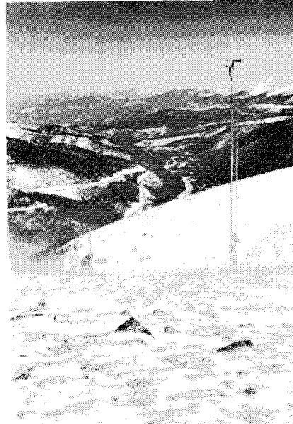
Figure 2. Project scientist, calibrating snow particle counter at the telemetry site on Colorado Mines Peak. Sensor is 50 cm aboveground; top of blowing snow layer is slightly above sensor. Windspeed and direction sensors are 10 m aboveground and 3804 m above sea level. Northward view shows Berthoud Pass highway, Fraser River valley, and west flank of Colorado's Front Range.
