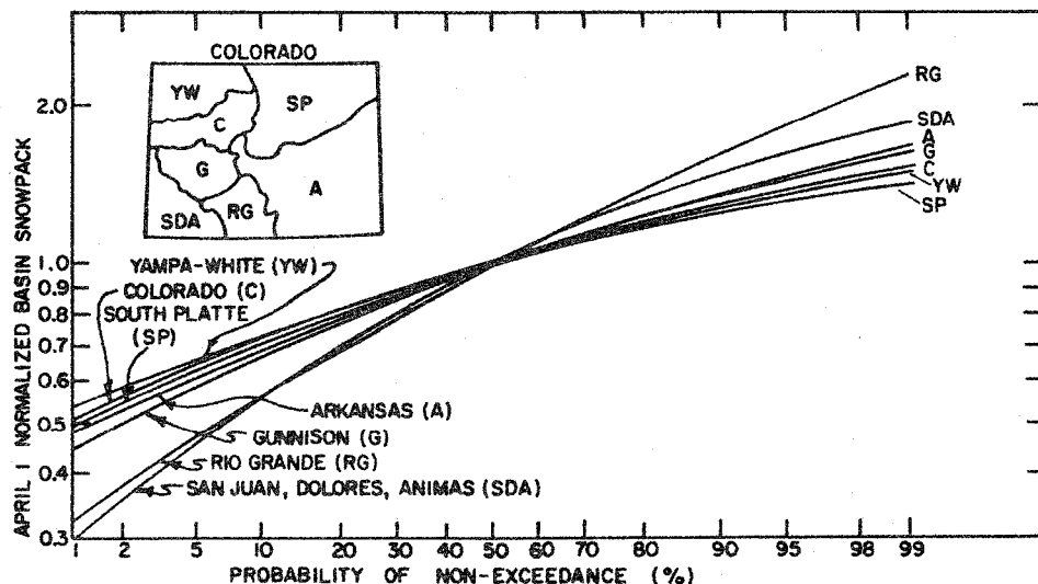
Figure 1. Frequency analysis of April 1 basin snowpack snow water equivalent (SWE) normalized to the median value.
