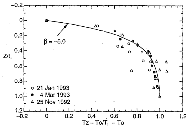
Figure 7. Nondimensional profiles at Well 8.
