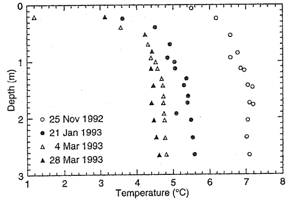
Figure 3. Temperature profiles at Well 8.
