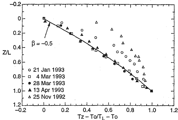
Figure 6. Nondimensional profiles at Well 1.
