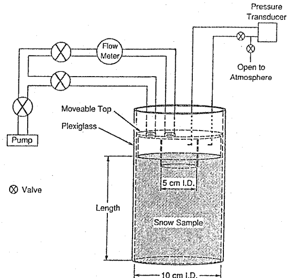
Figure 1. Schematic of air permeameter (after Chacho and Johnson, 1987).
