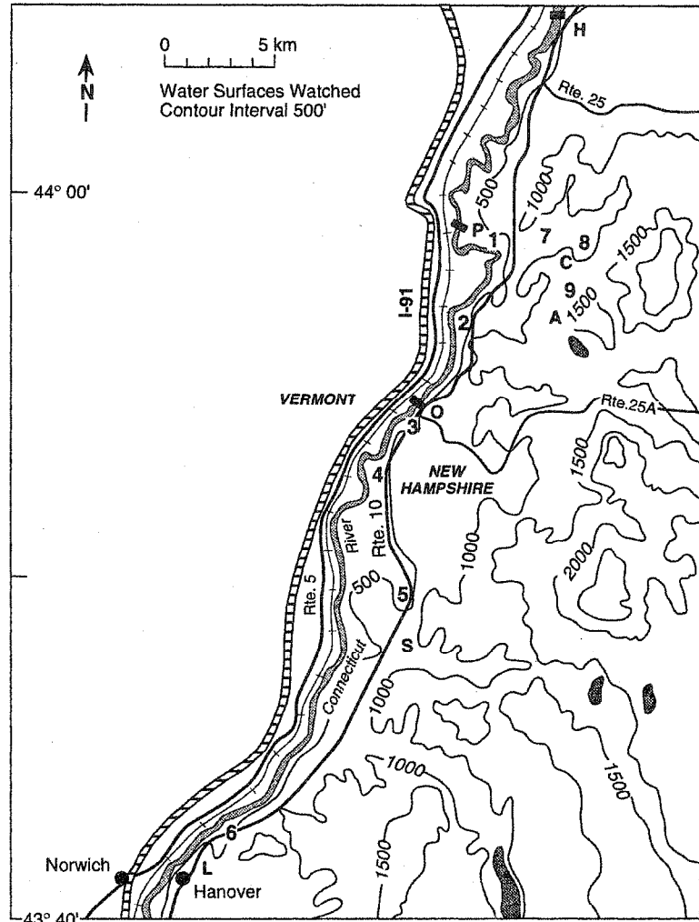
Figure 1. Connecticut River valley experiment area. Three bridges where over river temperatures were obtained are designated by H, P, and O. Basins of essentially equal elevation along the river are designated by 1, 2, 3, 4, 5, and 6. A narrow V-shaped valley along a brook is at 7, and two basins lie at 8 and 9, well above river level. The measuring point of greatest elevation is at A, and C designates the location of quantitative daily snow depth measurements. Other designated points are defined in the text.
