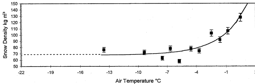
Figure 3. Relationship between new-fallen snow density and temperature (compilation of data reported by the US Army Corps of Engineers (1956) and Schmidt and Gluns (1991)). 95% confidence intervals shown along with means.
