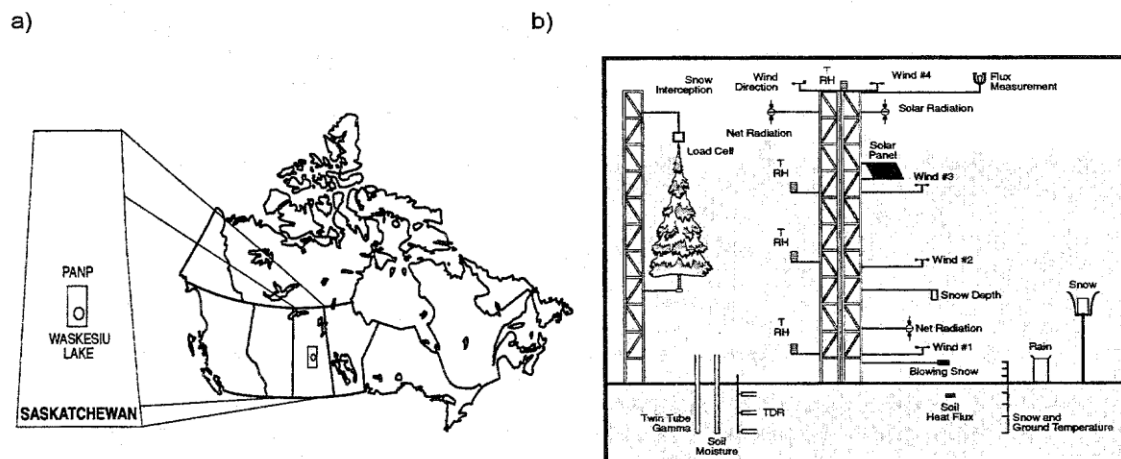
Figure 1. a) Experimental site location, b) Tower design and instrumentation. The schematic conceptualizes the basis for the towers used at the jack pine and black spruce sites.
