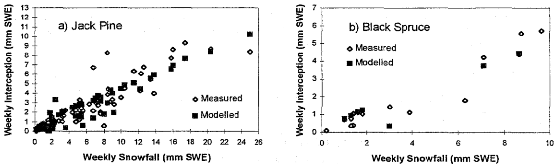
Figure 6. Comparison of modelled and measured weekly interception, a) jack pine, b) black spruce.
