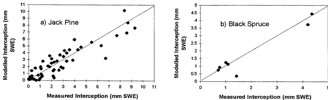
Figure 7. Modelled versus measured interception, a) jack pine coefficient of determination r^2 = 0.82 and standard error of estimate = 1.01, b) black spruce coefficient of determination r^2 = 0.92 and standard error of estimate = 0.51.
