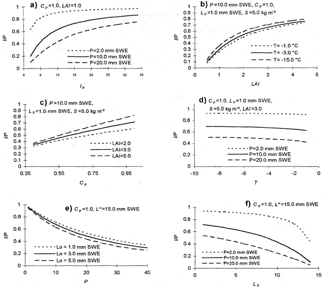
Figure 5. Sensitivity of modelled interception efficiency to input variables, a) storage capacity, b) leaf area index, c) canopy coverage, d) temperature, e) snowfall, and f) initial canopy snow load.
