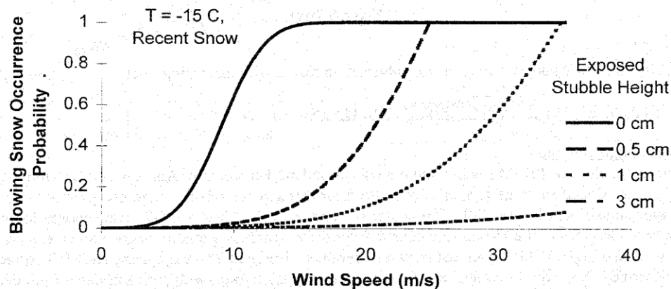
Figure 4. Probability of blowing snow over snowpacks with exposed cereal stubble stalks.
