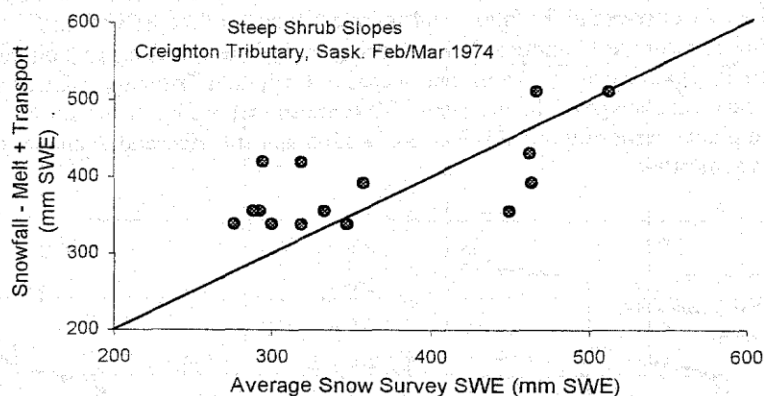
Figure 9 Estimated and measured accumulation for steep shrub-covered slopes, Creighton Tributary, Sask.
