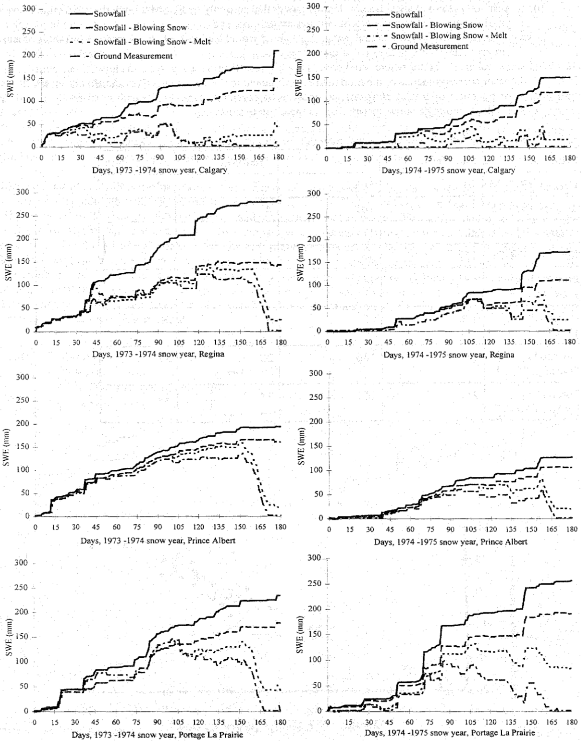
Figure 6 Simulated blowing snow fluxes, snow melt and surface snow mass balance and estimated snowfall and snow water equivalent for Climate Stations in the Prairie Provinces of Canada. Model simulations assumed fetch=1 km with short vegetation.
