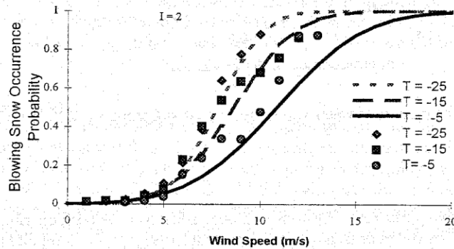
Figure 3. Blowing snow occurrence probability as a function of wind speed and air temperature for a snowpack 7 hours old: model and measurements
