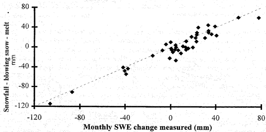
Figure 7. Monthly fluxes of snowcover mass balance by PBSM and changes in estimated snow water equivalent for 4 prairie climate stations over 2 years.
