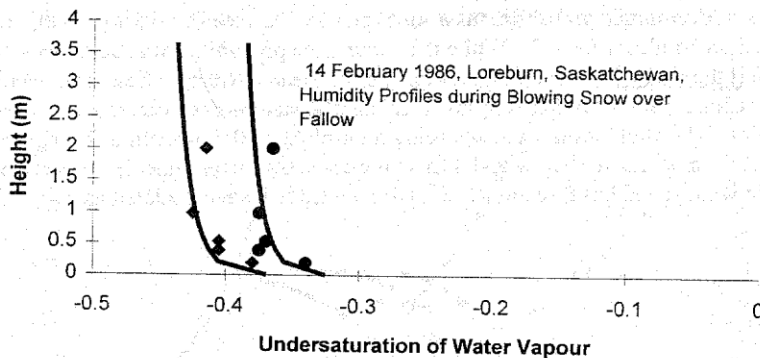
Figure 2. Vertical profiles of undersaturation of water vapour measured at Loreburn, Sask. during strong blowing snow, and modelled profiles.
