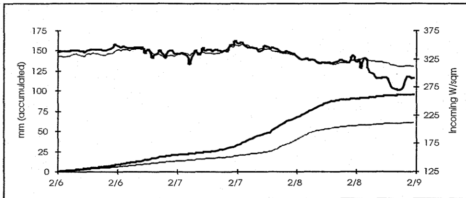
Figure 2a. Accumulated snow outflow and incoming longwave radiation during ROS event in Umpqua National Forest, 1996. (Heavy line is shelterwood, thin line is mature)
