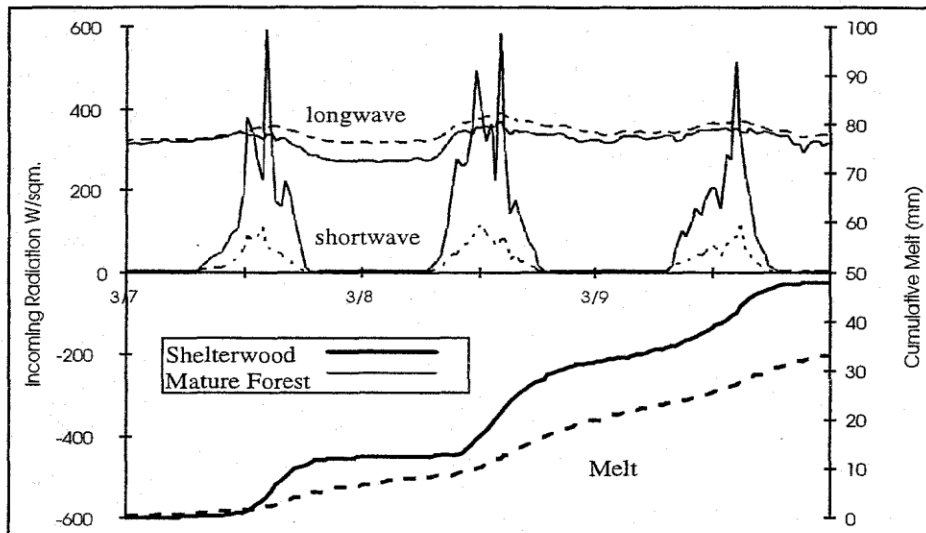
Figure 4. Accumulated outflow and incoming radiation during spring snowmelt event in the Umpqua National Forest, 1996. Dashed line is mature, Solid line is shelterwood
