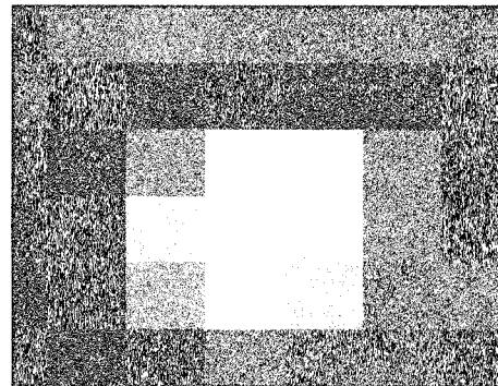
Fig. 1(b). Finger Mesa as seen by AVHRR
