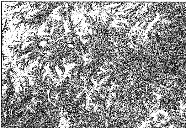
Fig. 1(a). Location of Finger Mesa (rectangle) inside the Upper Rio Grande Basin at Del Norte
