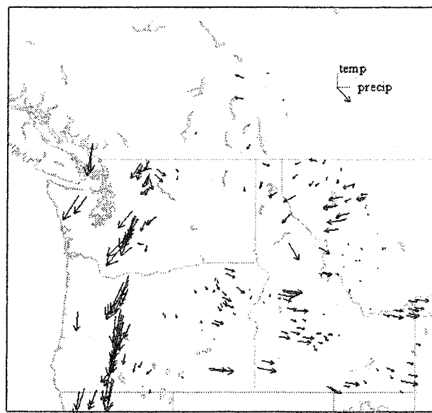
Figure 2. For each location, the arrow shows the trend in April 1 SWE attributed by multiple linear regression to precipitation \langle S \rangle_p (x-direction) and temperature and \langle S \rangle_T (y-direction). The reference arrow in the legend has a length of 10 cm of SWE.
